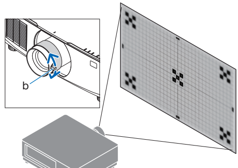
b: Fokushebel
