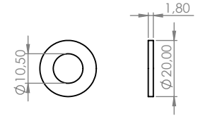
M10 flat washer
