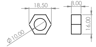
M10 Hexagonal nut
