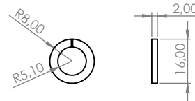
M10 spring lock washer
